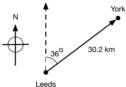
Figure: The distance from Leeds to York in geometric form
