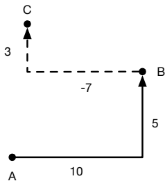
Figure: Vector Addition
